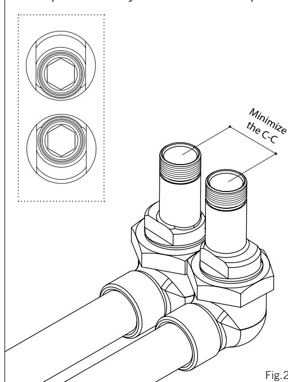
Correct position of asymmetrical hose adapters
